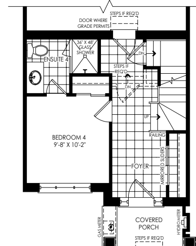
ELEVATION C, D OPT. 4 BEDROOM
