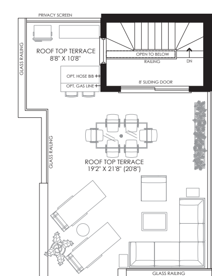
ROOF TOP TERRACE ELEV. 'K'
