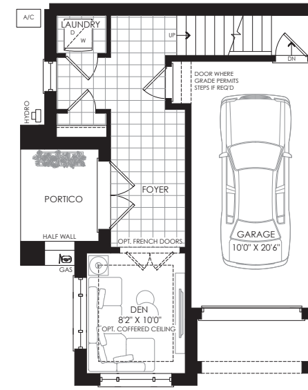
GROUND FLOOR PLAN ELEV. 'M'
