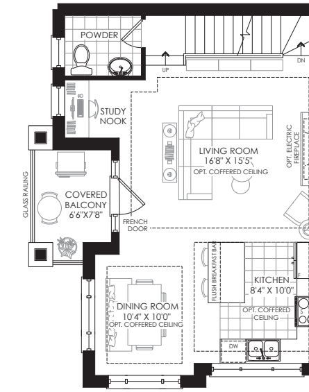
SECOND FLOOR PLAN ELEV. 'M'
