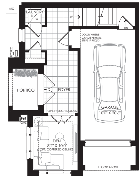
GROUND FLOOR PLAN ELEV. 'J'
