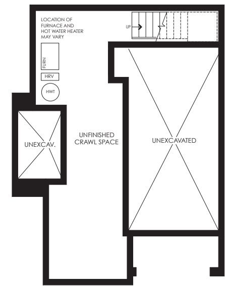
CRAWL SPACE PLAN ELEV. 'J', 'K', 'L' & 'M'
