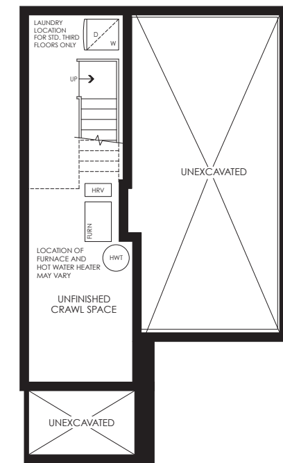
CRAWL SPACE PLAN ELEV. 'N','O'
