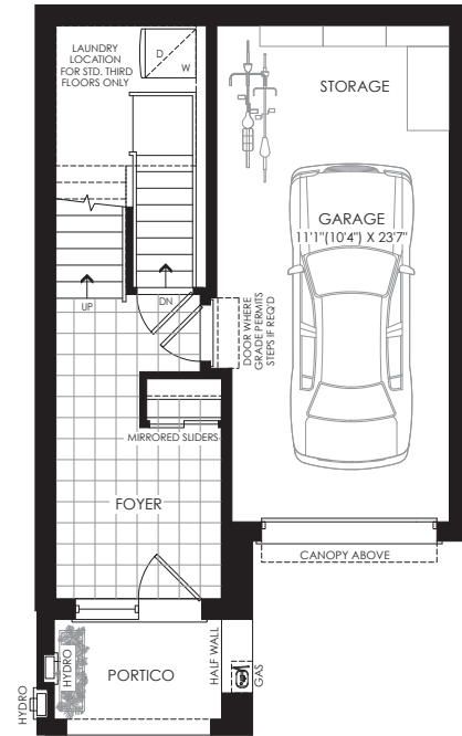
GROUND FLOOR PLAN ELEV. 'N','O'
