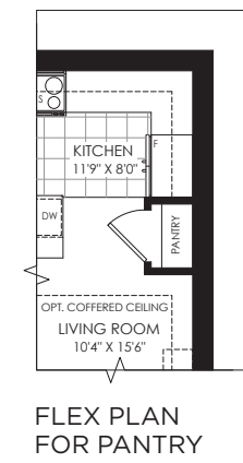
SECOND FLOOR PLAN ELEV. 'N','O'
