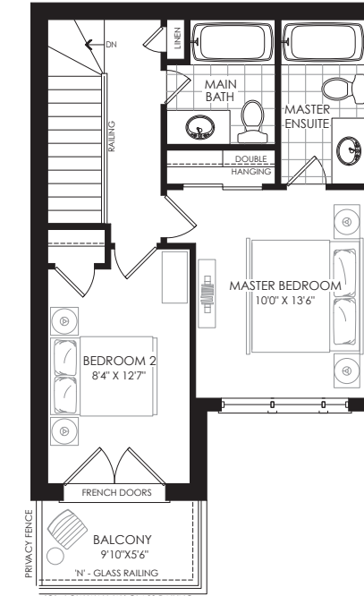
THIRD FLOOR FLEX PLAN ELEV. 'N','O' WITH MASTER ENSUITE
