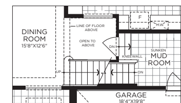
Basement & Main Floor - Flex (Fin. Basement Foyer)
