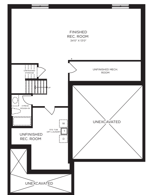
Finished Basement Floor Elev. A (Similar for Elevation B & C)
