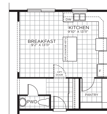
Main Floor - Flex (With Walk-in Pantry)
