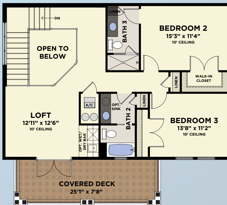
2ND FLOOR
