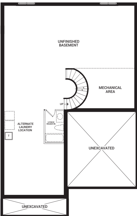
BASEMENT FLOOR PLAN A SIMILAR FOR PLAN B, C & D
